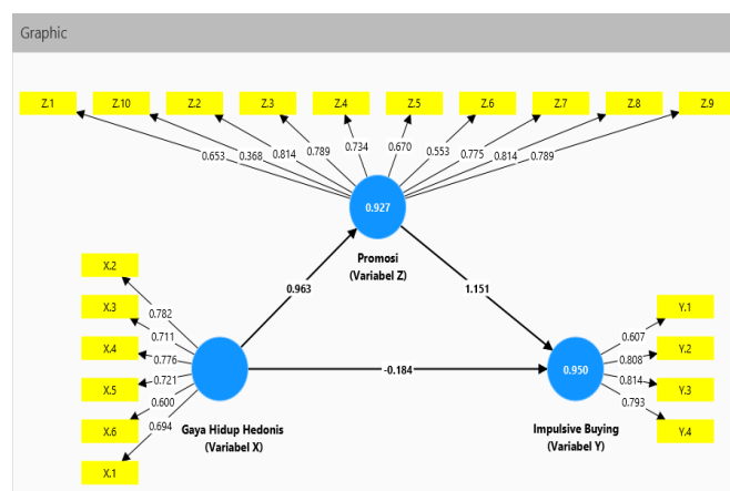
Gambar 2. Skema Model Partial Least Square (PLS)
