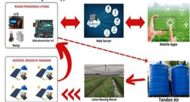
Figure 4. IoT work scheme in Shallot farming
